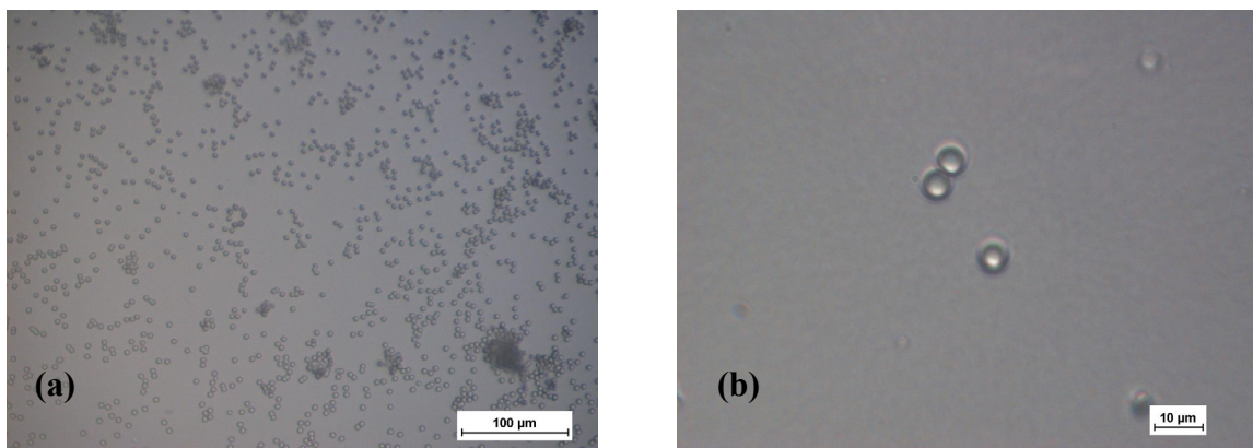
Fig. 8: 5 \mu m diameter silica spheres in water a) x20 b)x100.
