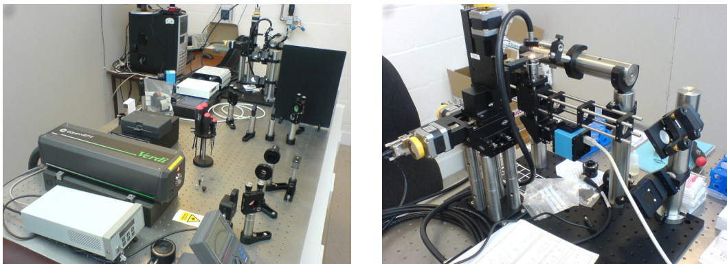
Fig. 4: NWLEC's optical trapping facility
