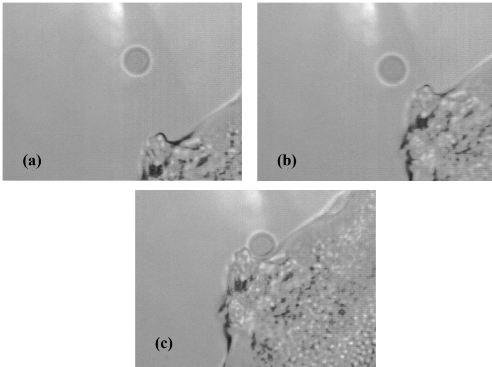
Fig. 10: Optical trapping sequence of a 5\mu\text{m} silica bead in water, \sim 100\text{mW} . Stronger filter in the camera allows the removal of the trapping laser from the image.
