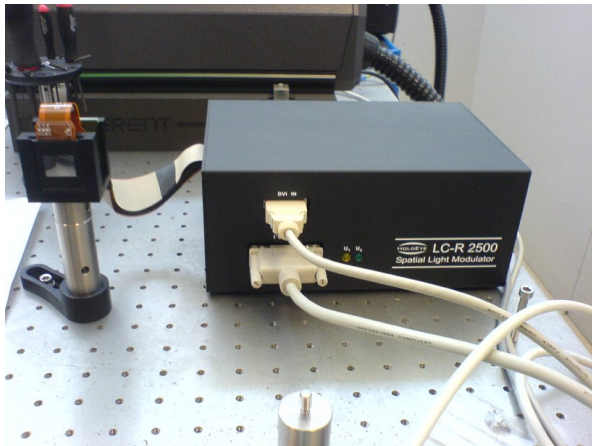
Fig. 2: Example of a Spatial Light Modulator (SLM). Holoeye LC-R 2500. This is a reflective element.
