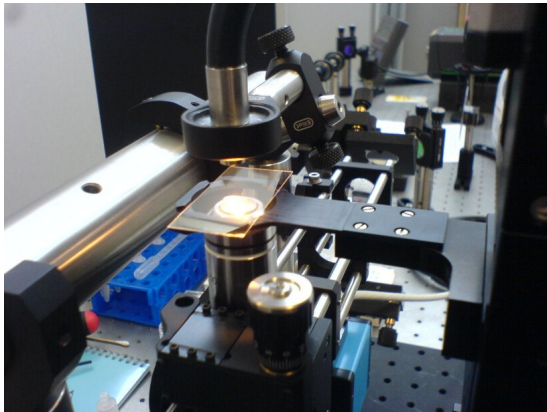
Fig. 7: Sample holding arm and illumination.
