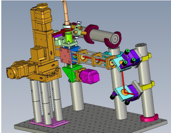
Fig. 5: Inverted optical tweezers design
