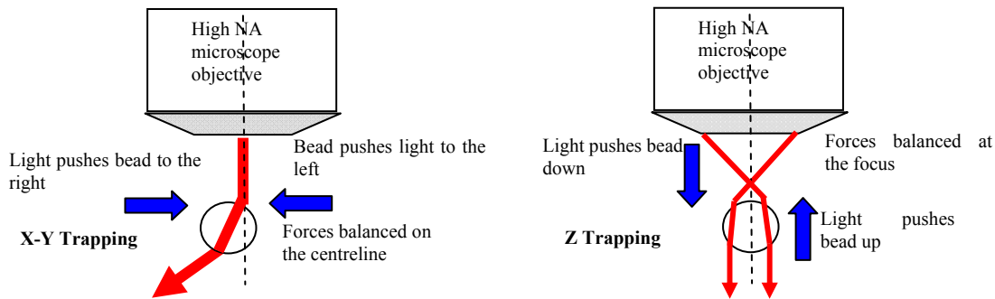
Fig. 1: Schematic of light-bead interaction that gives rise to optical trapping forces in a tightly focused Gaussian laser beam.
