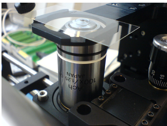
Fig. 6: High NA inverted microscope objective.
