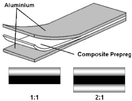
Fig. 1 Typical FML lay-ups
